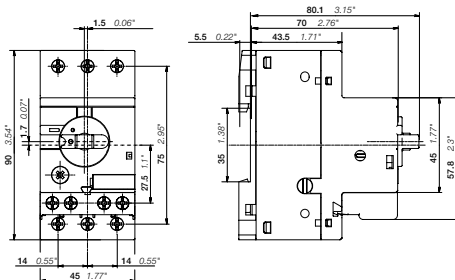
MS116 ≤ 16 A
