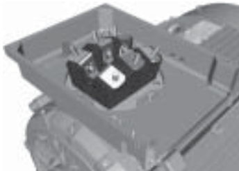
Terminal box for motor sizes 280 to 315, provided either with a cable gland or a cable box.
