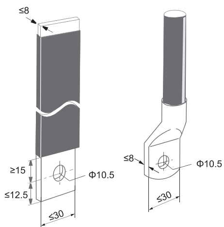
NM8N-400/630
